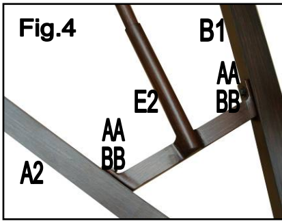
Fig.4: Attach E2 to the middle of Arc Pole 2 (A2) and B1 by M6X20 Bolt (AA) and M6 Washer (BB).
