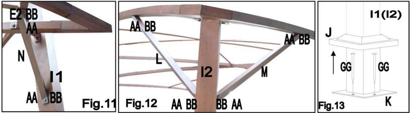
Fig.11: Attach Knighthead 3 (N) to Beam Connector 2 (E2) by M6X20 Bolt (AA) and M6 Washer (BB).
